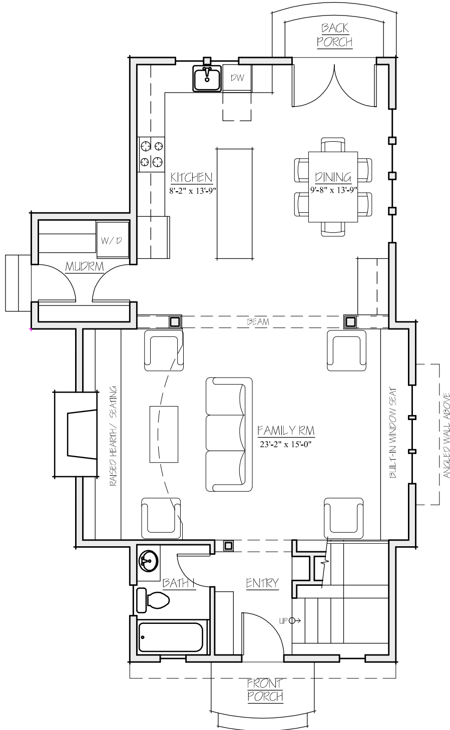
C101a: First level Floorplan
